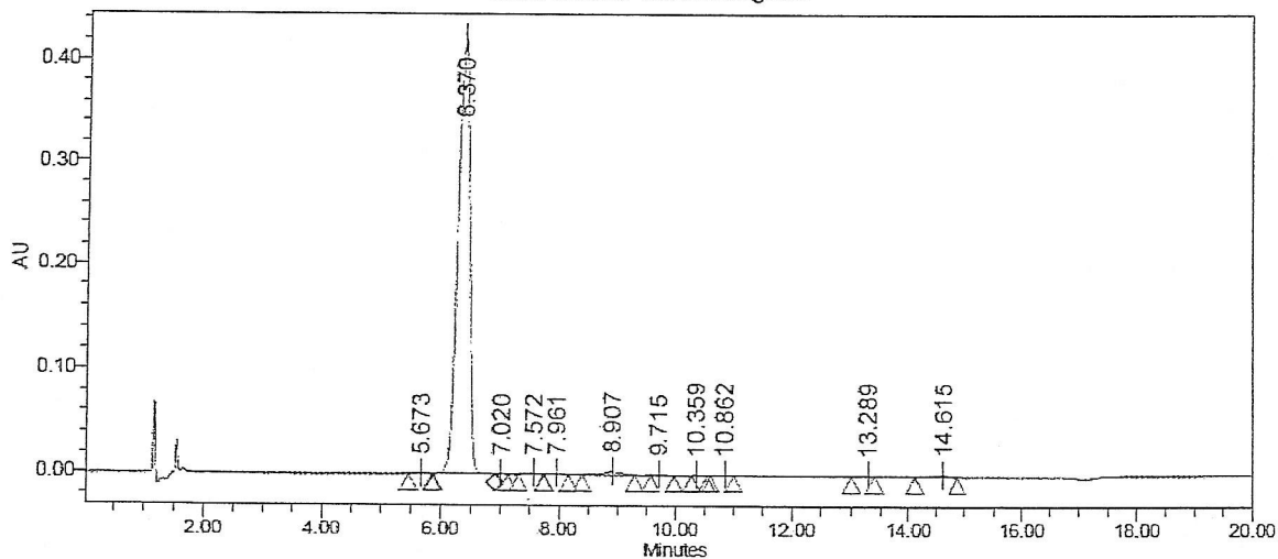
Auto-Scaled Chromatogram
